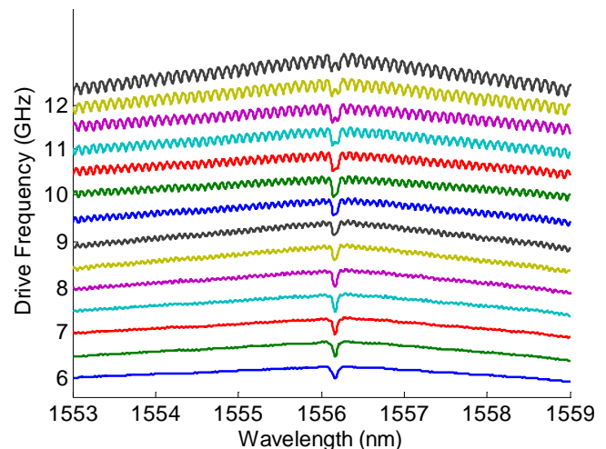
Fig. 10 The OCFG output optical spectra when the RF frequency is stepped from 6 GHz (lowest trace) to 12.5 GHz (top trace), at 0.5 GHz per step, at one second intervals. All comb spectra maintain a 6 dB power envelope of approximately 6 nm.
