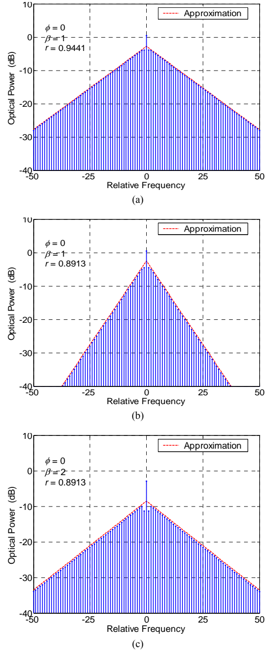
Fig. 1 Optical spectrum generated by the OFCG under different conditions
