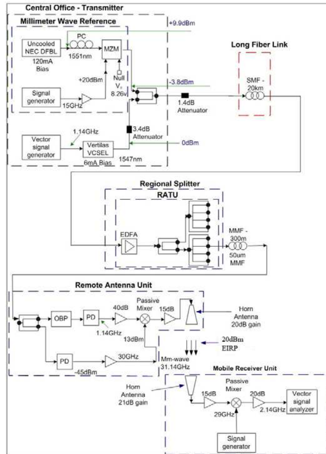
Fig. 2 - Downlink experimental setup including wireless path. Photodiode (PD), erbium-doped fiber amplifier (EDFA), Mach-Zehnder modulator (MZM), optical bandpass filter (OBP), single-mode fiber (SMF), multimode fiber (MMF), remote antenna termination unit (RATU), vertical-cavity surface-emitting laser (VCSEL), distributed feedback laser (DFBL), effective isotropic radiated power (EIRP)
