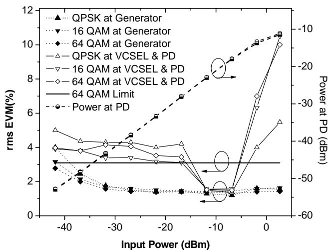
Fig. 4 – Average rms EVM and power measurement for WiMAX emulated schemes at 20MSps after the VCSEL and photodiode link (back to back) for different input power levels.
