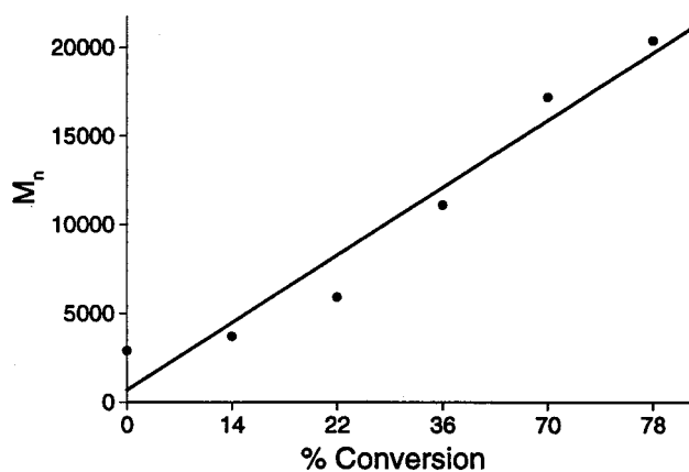
Figure 1. A plot of M_n versus % conversion for the synthesis of a low molecular weight graft copolymer (calculated \overline{DP} ~ 70).
