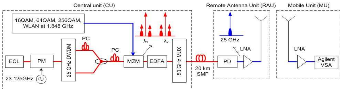
Fig. 3 Radio over fiber and wireless transmission experimental setup. ECL: External cavity laser, PM: Phase Modulator, PC: Polarization Controller, MZM: Mach Zehnder Modulator, EDFA: Erbium doped Fiber Amplifier, PD: Photodiode, LNA: Low Noise Amplifier
