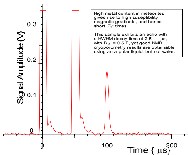
Fig. 3: NMR Spin-Echo from an a-polar liquid in a Meteorite sample ALH77307. Due to susceptibility gradients, the echo has a decay time HWHM of 2.5 \mu\text{s}
