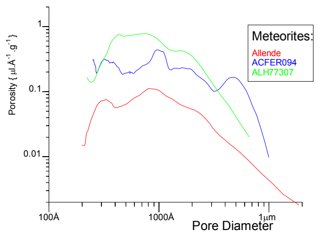
Fig. 4: Pore size distributions for 3 Meteorite samples, as measured by NMR cryoporometry, using an a-polar liquid.
