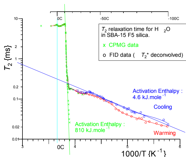
Fig 2. NMR relaxation rates T_2 for plastic ice in SBA-15 silica pores.
