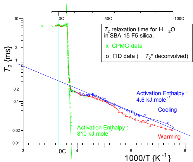
Fig 2. NMR relaxation rates T_2 for plastic ice in SBA-15 silica pores.
