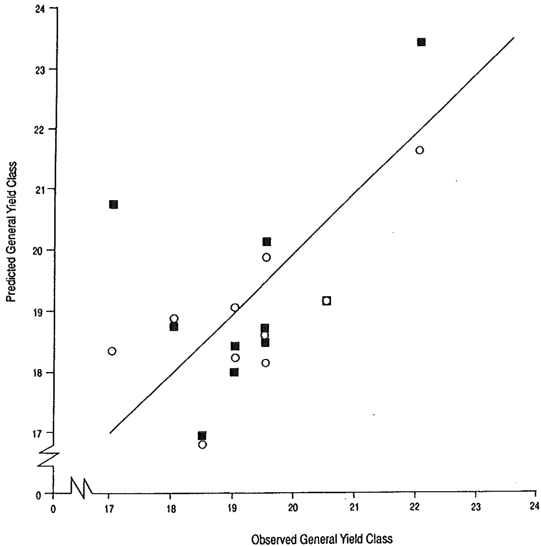
Figure 4: Plot of predicted against observed General Yield Class using an independent data set to validate this model (o) and MacMillan's model (■).
