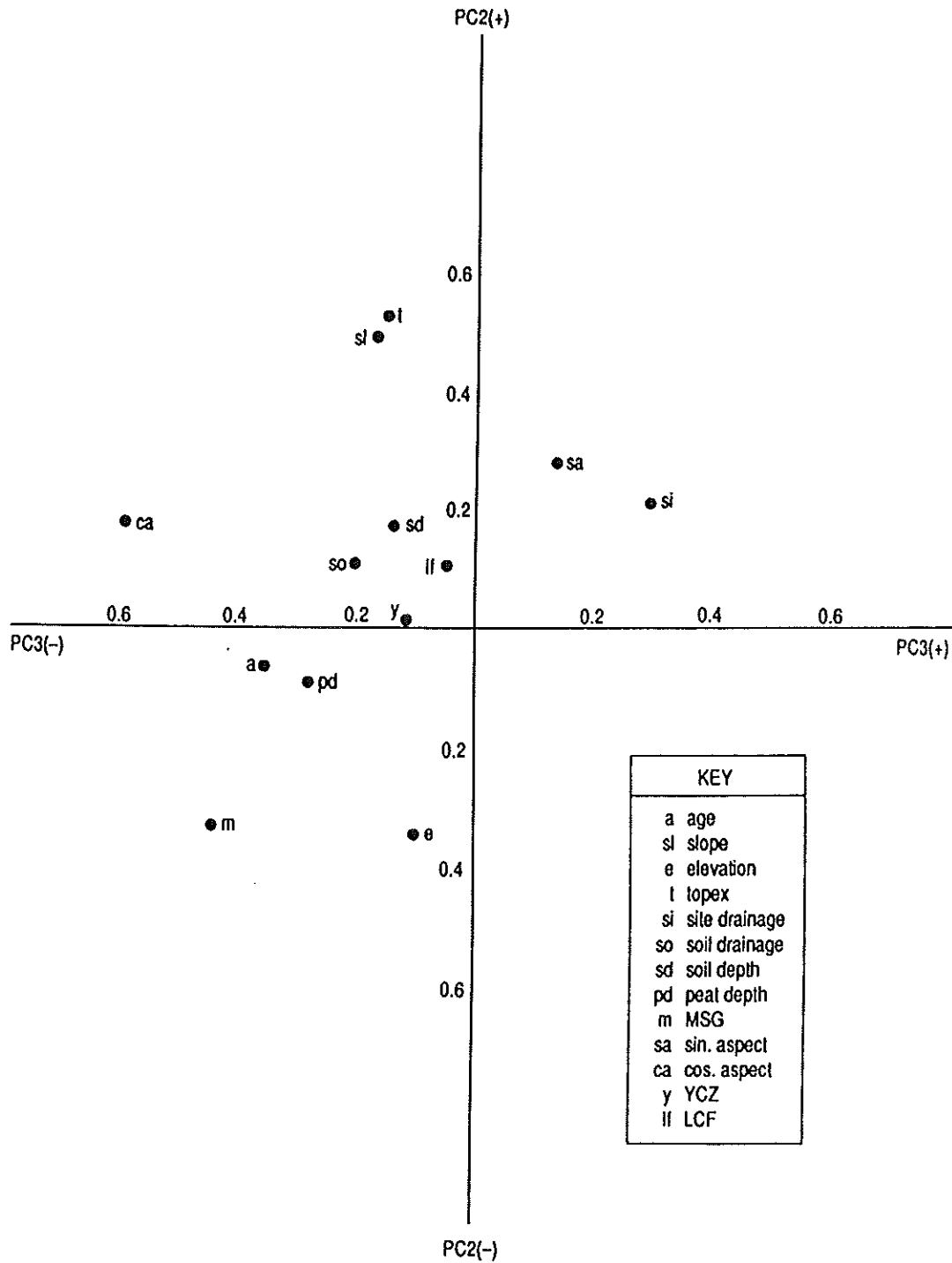
Figure 2: Plot of principal component load values for PC2 and PC3
