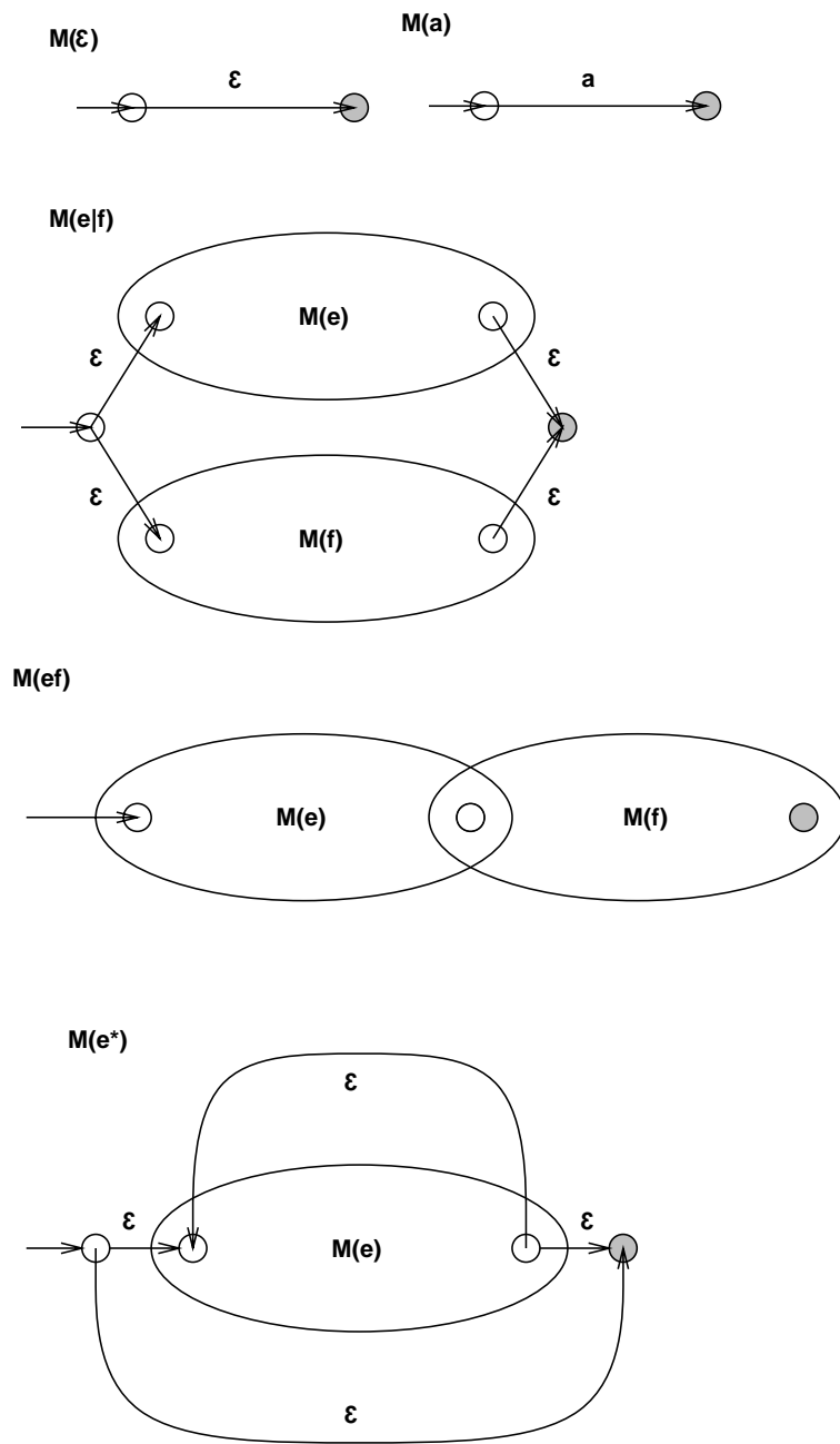
Figure 3: Building NFAs for regular expressions
