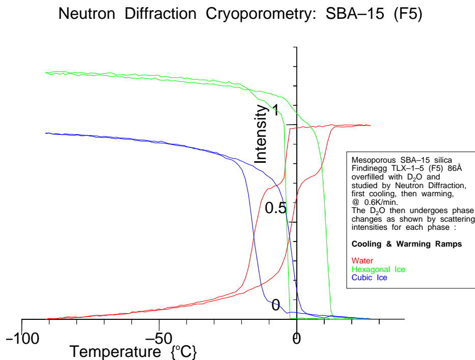
Figure 5. Neutron diffraction cryoporometric curves for ice/water freezing and melting in overfilled SBA-15 (F5) templated silica with a nominal pore diameter of 86Å, showing the separately resolved data for cubic ice, hexagonal ice and water.
