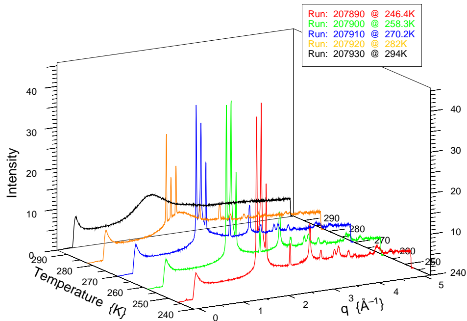
Figure 3. Neutron diffraction curves for the melting of ice to water in overfilled SBA-15 (F5) silica.
