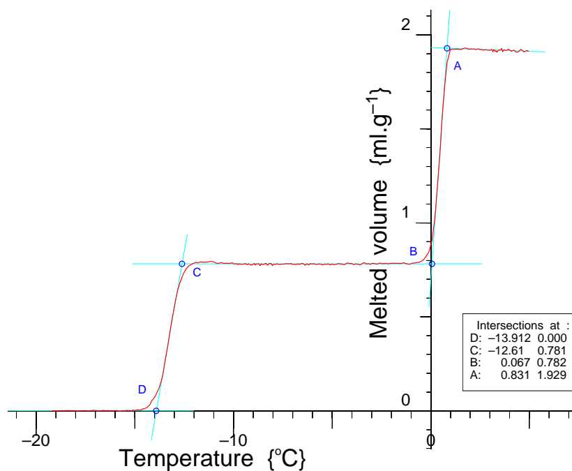
Figure 1. NMR cryoporometric melting curve for H 2 O in SBA-15 TLX-1-5 (F5) templated silica, at a warming rate of 0.05 C°.min -1 .
