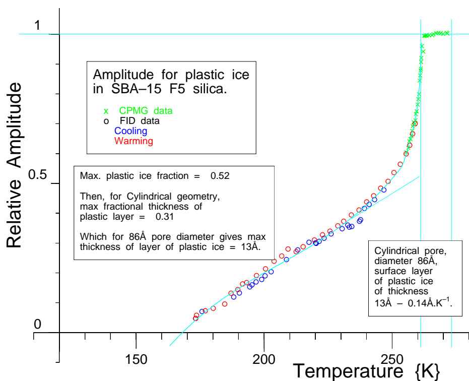
Figure 8. Amplitude of NMR signal for plastic ice in SBA-15.
