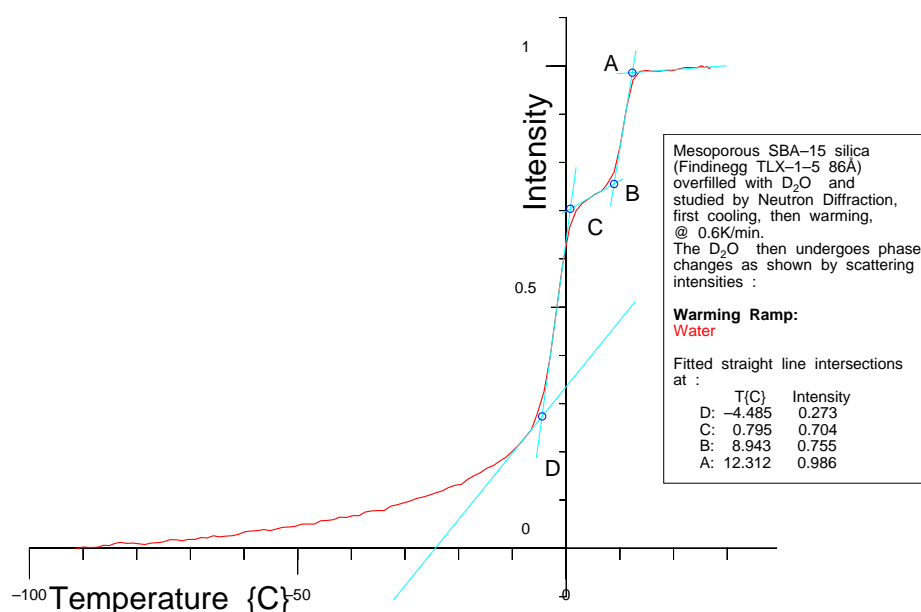
Figure 6. Neutron diffraction cryoporometry curves for water melting in overfilled SBA-15 (F5) templated silica with a nominal pore diameter of 86Å, showing disordered component between -80°C and -5°C.
