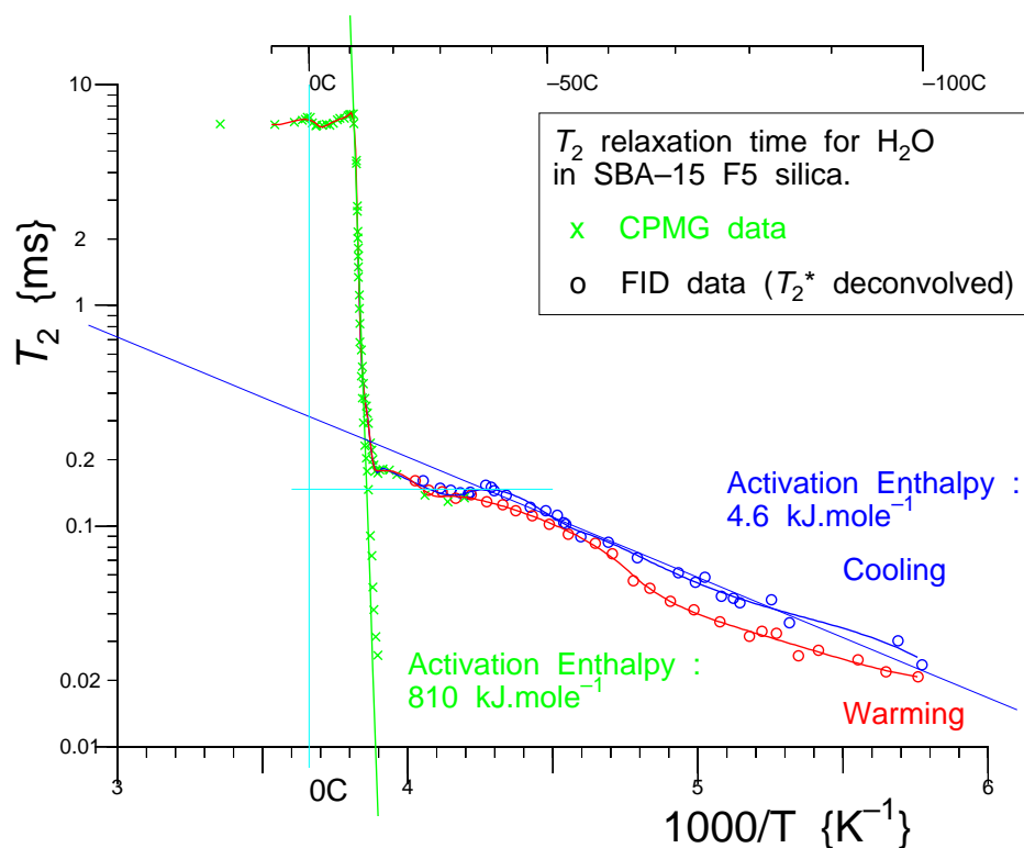
Figure 9. Variation with temperature of the long T_2 relaxation time component for plastic ice in SBA-15 porous silica - Arrhenius plot.
