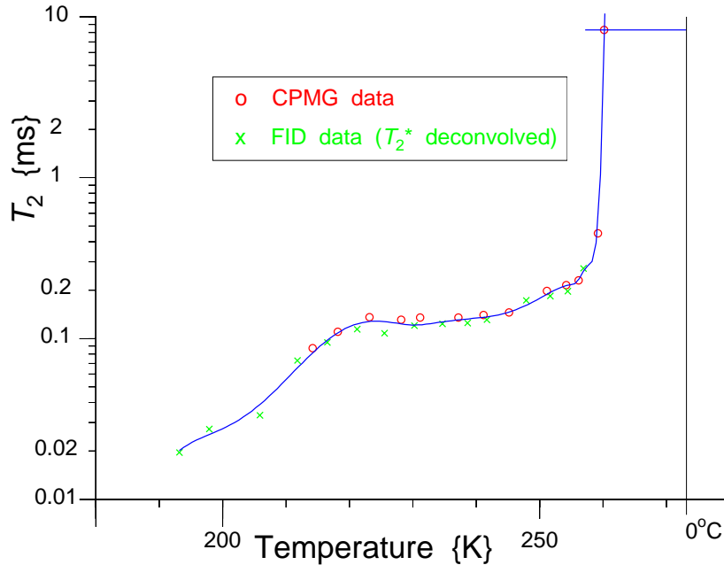
Figure 8. The variation in the NMR proton T_2 relaxation time as a function of temperature for water/ice in SBA-15.
