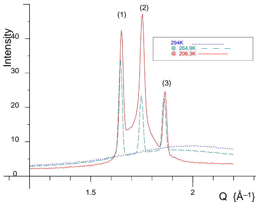
Figure 5. A selected set of intensity profiles for the water, hexagonal and cubic ice peaks.
