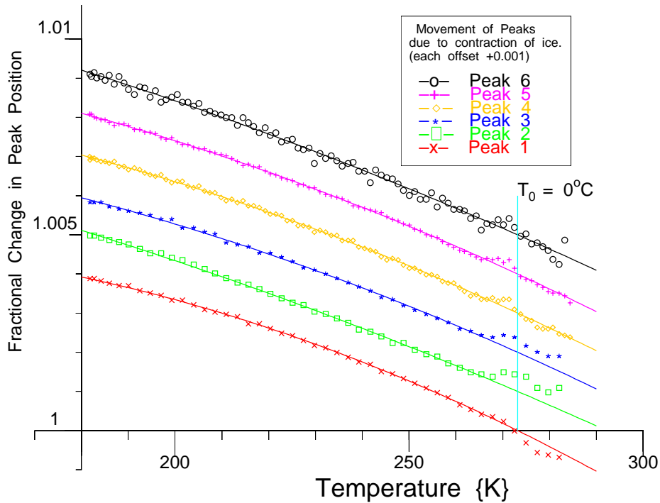
Figure 7. The relative variation of the various peak positions as a function of temperature; the fitted lines are for equation 8 with parameter given in table 2.
