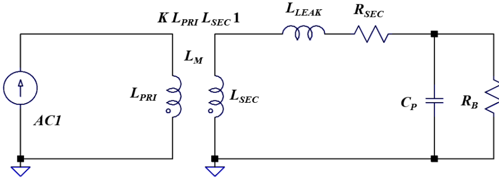
Fig. 3. Simplified HFCT equivalent lump circuit model for parameter measurement.
