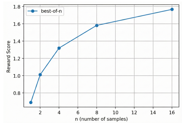
Figure 8: Reward Score using Best-of- n for Gemini 2.5 Pro.
