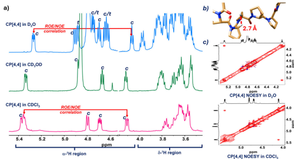
FIGURE 2 | (a) ^1\text{H} -NMR of CP[4,4] in \text{CDCl}_3 , \text{CD}_3\text{OD} , and \text{D}_2\text{O} . Only the all-junctions- cis isomer is observed in \text{CDCl}_3 and \text{CD}_3\text{OD} , whereas a mixture of all-junctions- cis and all-junctions- trans is observed in \text{D}_2\text{O} . All \alpha -protons of CP[4,4] are marked with c for the all-junctions- cis conformation or t for the all-junctions- trans conformation. ROE/NOE correlations between the L/D junction points are highlighted; (b) SC-XRD of all-junctions- cis CP[4,4] highlighting the distance between the two \alpha -protons at the L- and D-proline junctions; (c) zoomed-in region of the CP[4,4] NOESY spectrum in \text{D}_2\text{O} and \text{CDCl}_3 .
