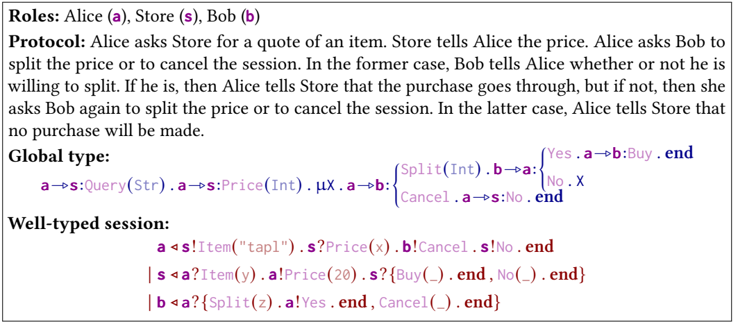
(b) Recursive Two-Buyers
