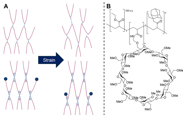
Fig. 21 (A) Schematic overview of crosslinked polymers versus slide-ring polymers and their differing response to strain. (B) The structure of the supramolecular elastomer, PACγCDAAMe produced by Nomimura et al. 196
