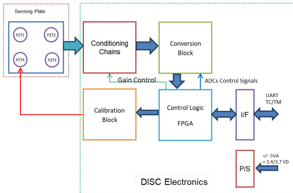
Fig. 2. DISC electronics functional blocks diagram.
