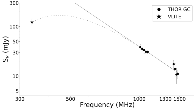
Figure 3. Stokes I flux density of ASKAP J173608.2–321635 from THOR-GC and VLITE observations on 2020 April 11. A power law relation ( S_\nu \sim \nu^\alpha ) is fitted (solid) to the THOR-GC data with \alpha = -3.1 \pm 0.2 . A power law relation with free-free absorption is fitted (dashed) to the combined THOR-GC and VLITE data with \alpha = -3.6 \pm 0.3 and \tau = 0.4 \pm 0.06 at 1 GHz.
