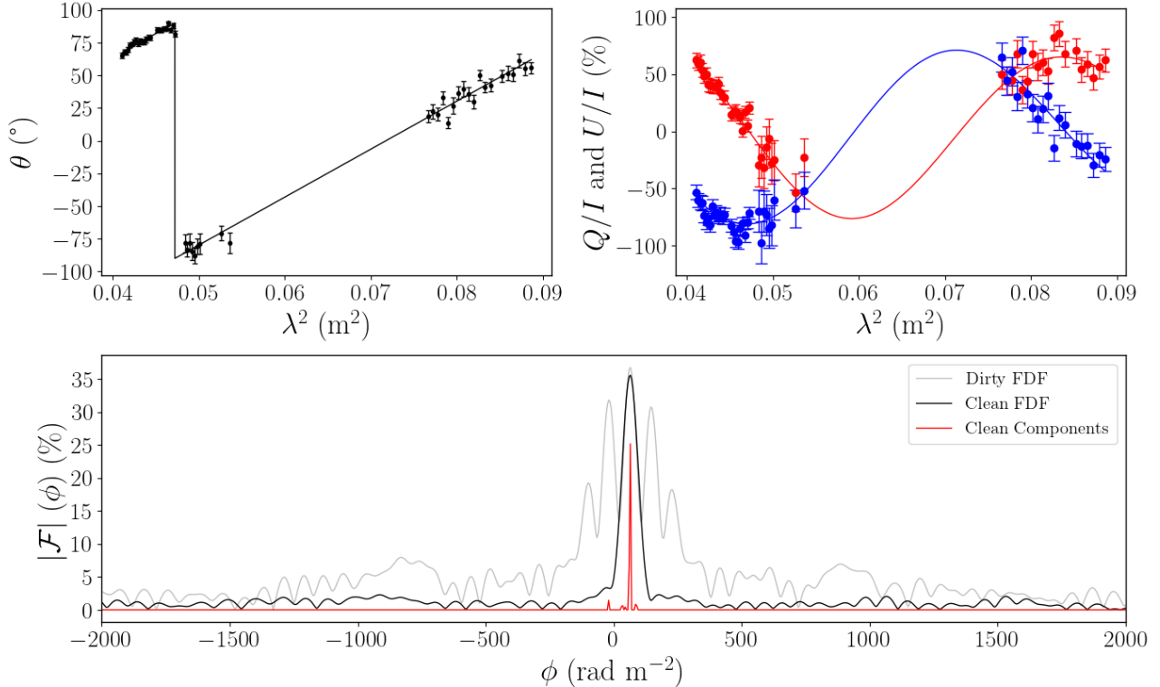
Figure 4. Results of QU fitting and RM clean for ASKAP J173608.2–321635 for the detection in THOR-GC on 2020 April 11. The top left panel shows polarization angle as a function of \lambda^2 with the model from QU fitting. The top right panel shows Stokes Q (blue) and U (red) as a function of \lambda^2 with the result of QU fitting indicated by the solid lines. The bottom panel shows the dirty Faraday dispersion function (FDF) in gray, clean FDF and RM in black and clean components from RM clean in red.
