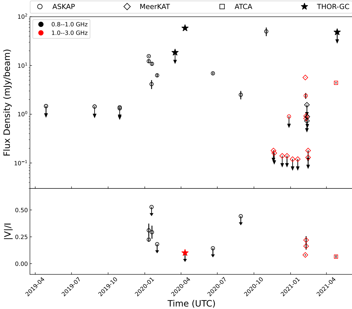
Figure 1. Flux density of ASKAP J173608.2–321635 as a function of time (adapted from Wang et al. 2021). The ASKAP, MeerKAT and ATCA flux densities are from Wang et al. (2021). The colour of the symbols indicates the same broad frequency ranges as in Wang et al. (2021). Arrows indicate 3\sigma upper limits. THOR-GC total flux densities and upper limits have been extrapolated to 900 MHz assuming a spectral index of \alpha = -3.1 . The THOR-GC circular polarization upper limits is for \nu = 1.23 GHz (Table 1). The bottom panel shows fractional circular polarization of the source.
