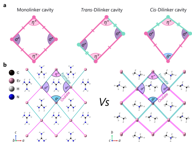
Fig. 1: a Unique cavity geometries generated by the introduction of distinct linker types and their respective orientation. Lithium L-tartrate is a rare example of a system with NLC with a trans -dilinker cavity. 14 b The winerack structures of (left) [\text{C}(\text{NH}_2)_3]\text{Er}(\text{HCO}_2)_2(\text{C}_2\text{O}_4) and (right) [(\text{CH}_3)_2\text{NH}_2]\text{Er}(\text{HCO}_2)_2(\text{C}_2\text{O}_4) with the organic struts reduced to Er–Er distances, in green for formate linkers and pink for oxalate linkers. The internal angles of the cavities highlight the unique cis -dilinker geometry.
