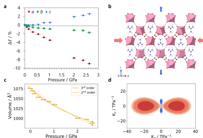
Fig. 2: a The change in lattice parameters of GUA with pressure, b the winerack structure of the framework, showing the directions of expansion (blue arrows) and contraction (red arrows) with applied pressure viewed along b , c The reduction in volume with increasing pressure, fit with a 3 rd order Birch–Murnaghan equation of state to extract B_0 , and d the indicatix tensor where the compressibility constants are negative (blue) and positive (red) and with the plotted eigenvalues calculated using PASCAL. 6
