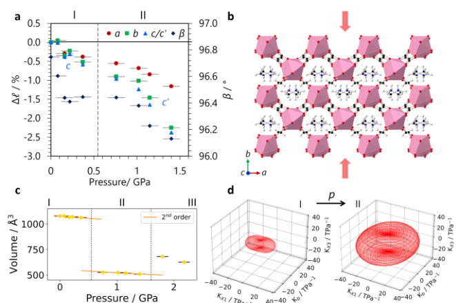
Fig. 3: a The change in lattice parameters of DMA with pressure and the phase I to II transition indicated by a dotted line. The lattice parameters of phase II have been normalised for direct comparison with phase I where in phase II c' = 2c . b The structure of DMA at ambient pressure with compression along b highlighted by red arrows. c The 2 nd order Birch–Murnaghan equations of state fits giving B_0 = 23(5) GPa for phases I and B_0 = 13(4) GPa for II. d The indicatrix tensors highlighting the change in compression between phase I, between 0 GPa - 0.37(10) GPa and phase II, between 0.76(10) GPa - 1.40(10) GPa.
