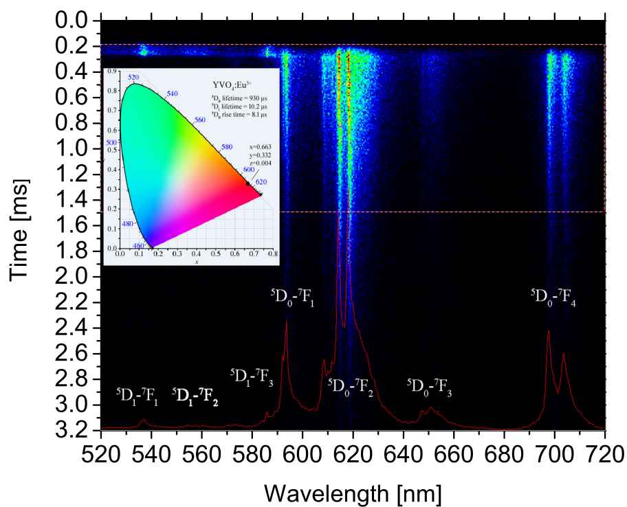
Fig. 6 Typical time-resolved spectrum of rare earth doped phosphor (YVO 4 :Eu) acquired in our measurements. Europium transitions are denoted. Inset shows CIE plot (color coordinate diagram) calculated from spectral data.
