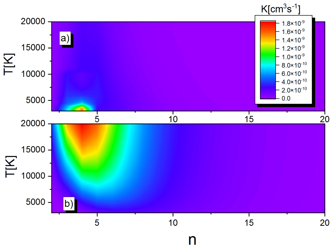
Fig. 4 a) Rate coefficient for associative ionization channel (upper) of eqn 1 as a function of n and T for the case X = \text{H} . b) same as a) but for non-associative ionization channel (lower) of eqn 1. Dataset is obtained in Srećković et al. 54
