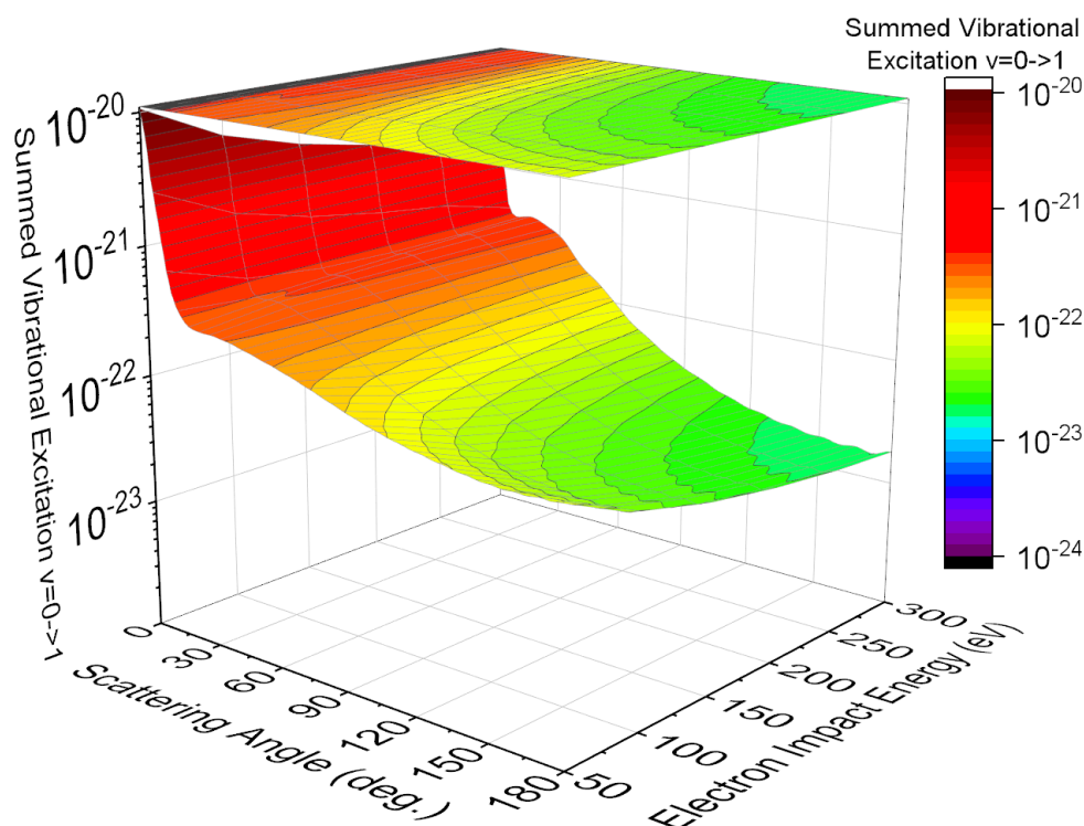
Fig. 2 Sum of 21 modes for rotationally summed 0→1 vibrationally inelastic absolute differential cross sections for scattering of electrons by furan molecule, calculated by UFBA method. The dataset is presented in Maljković et al. 33 .
